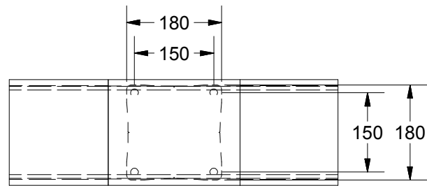
DETAIL B SCALE 1/10 MID POST
