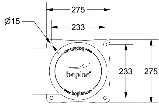
DETAIL A SCALE 1/10 END POST
